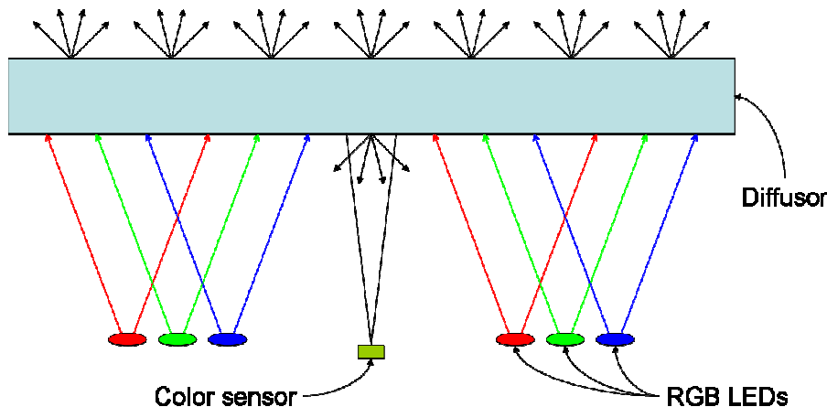
Figure 3: Color sensor placed in a LED system
